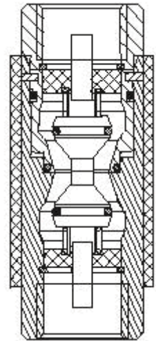
Construction of Breakaways
