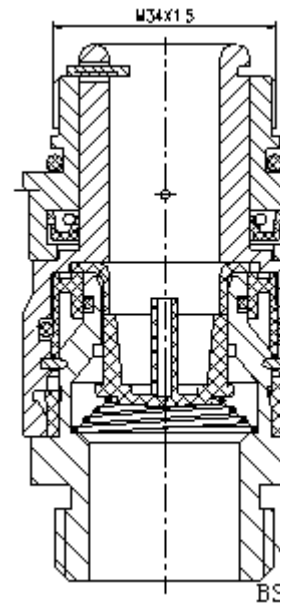
Construction of MD-5-11 Breakaway
