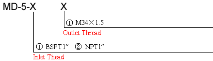
Construction of MD-5-11 Breakaway
